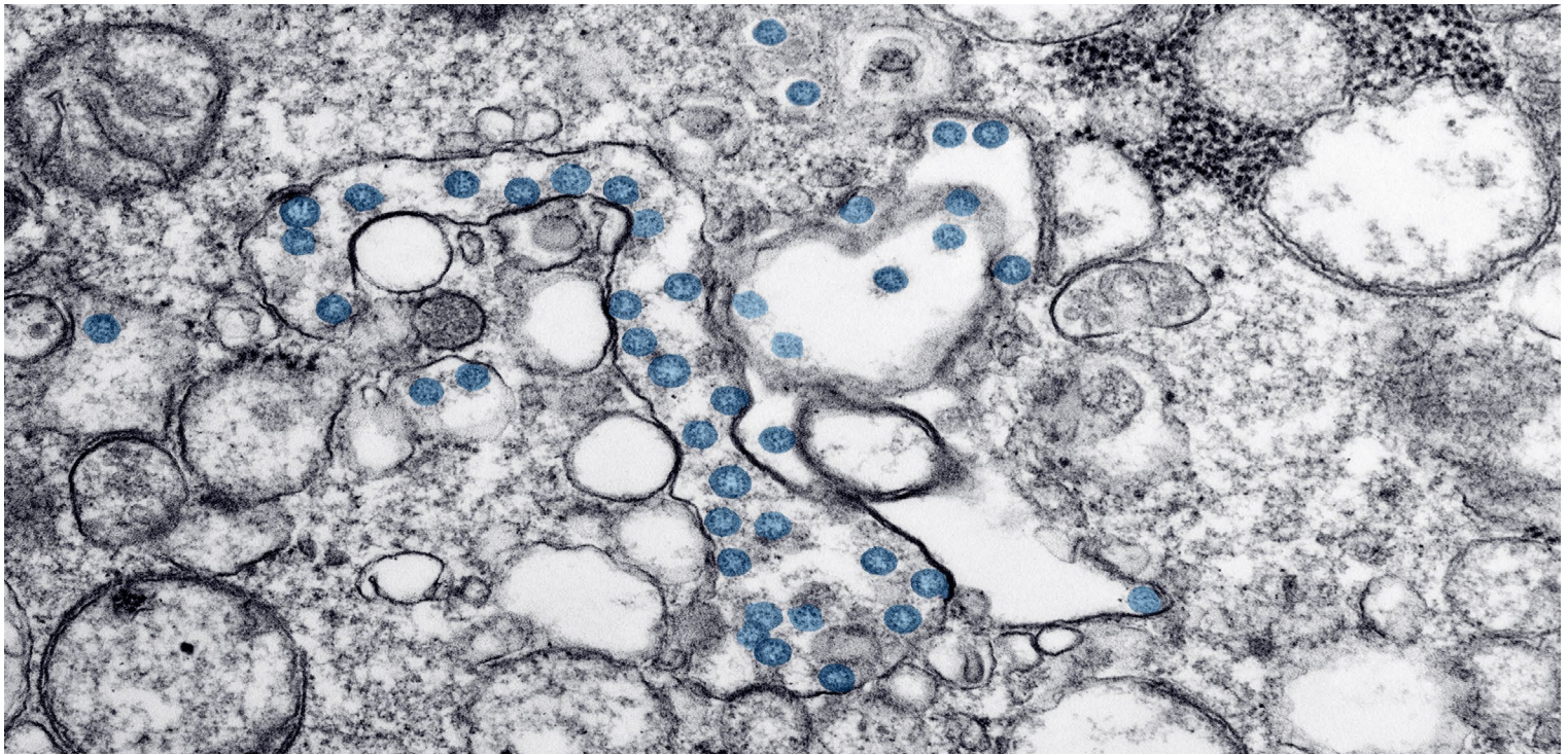
Transmission electron microscopic image of an isolate from the first US case of COVID-19. The spherical viral particles, coloured blue, contain cross-sections through the viral genome, seen as black dots. Photo credit: Hannah A Bullock and Azaibi Tamin/ Public Health Image Library (PHIL), Centers of Disease Control and Prevention (CDC)
