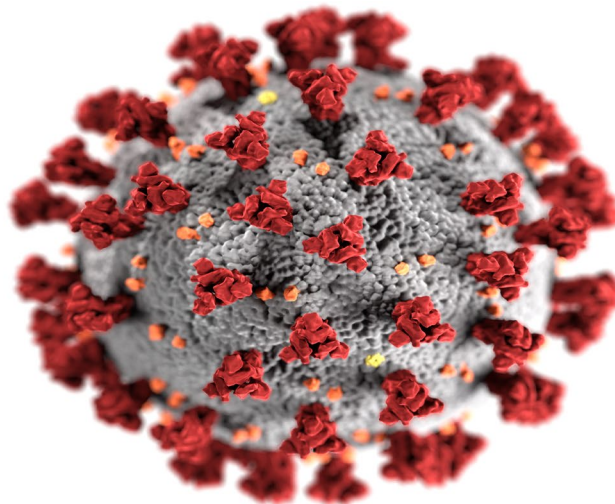
Ultrastructural morphology exhibited by coronaviruses. The red spikes look like a corona surrounding the virion when viewed electron microscopically. Photo credit: Alissa Eckert and Dan Higgins/PHIL/CDC
