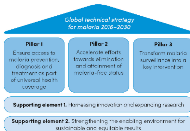
Figure 1: Global technical strategy for malaria 2016 - 2030: framework, pillars and supporting elements
